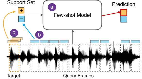
Fig. 1. Proposed few-shot sound event detection method. To detect a target sound event in a recording, we (a) apply metric-based few-shot learning, (b) automatically construct a set of negative (blue) examples needed for inference, and (c) propose an inference-time data augmentation method to generate more positive examples (orange).
