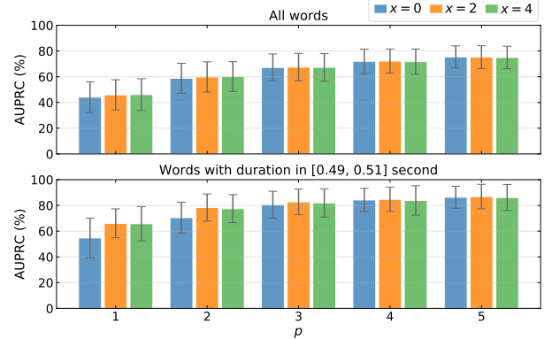
Fig. 5. AUPRC results for different p and x . Results are from the best model: Prototypical Networks with (C, K, n) = (10, 5, \text{All}) . (Top) All target keywords are tested. (Bottom) Only keywords with duration close to half-second context window are considered.
